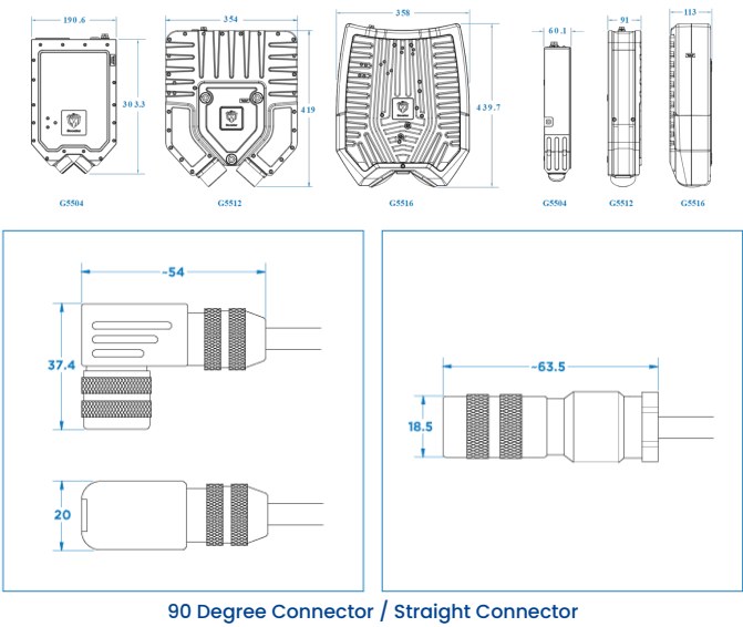
90 Degree Connector / Straight Connector
